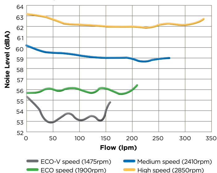
Hydrostorm ECO-V 100 Noise Levels
