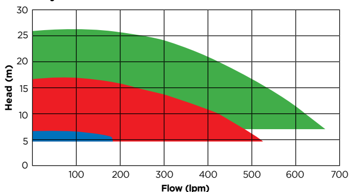
Hydrostorm ECO-V 300 Performance Curves
